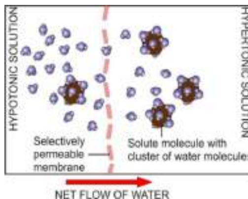
Figure 3.36: Osmosis at molecular level
